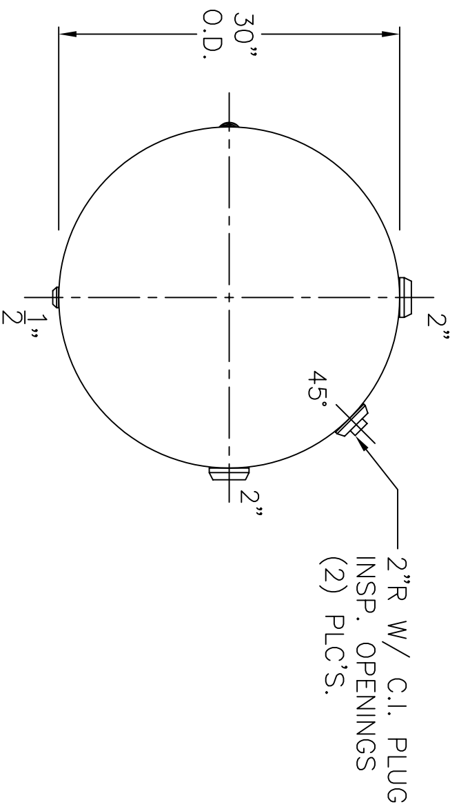
VIEW W/O SUPPORTS
