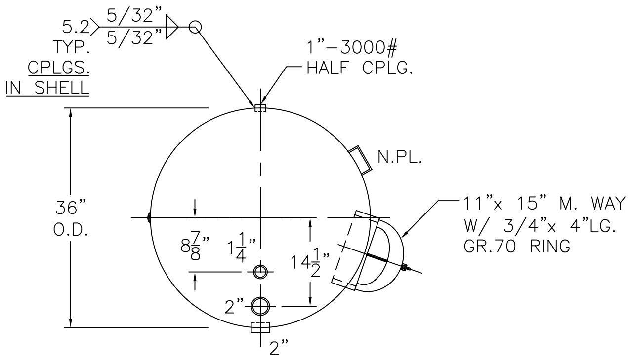
END VIEW W/OUT SUPPORTS
