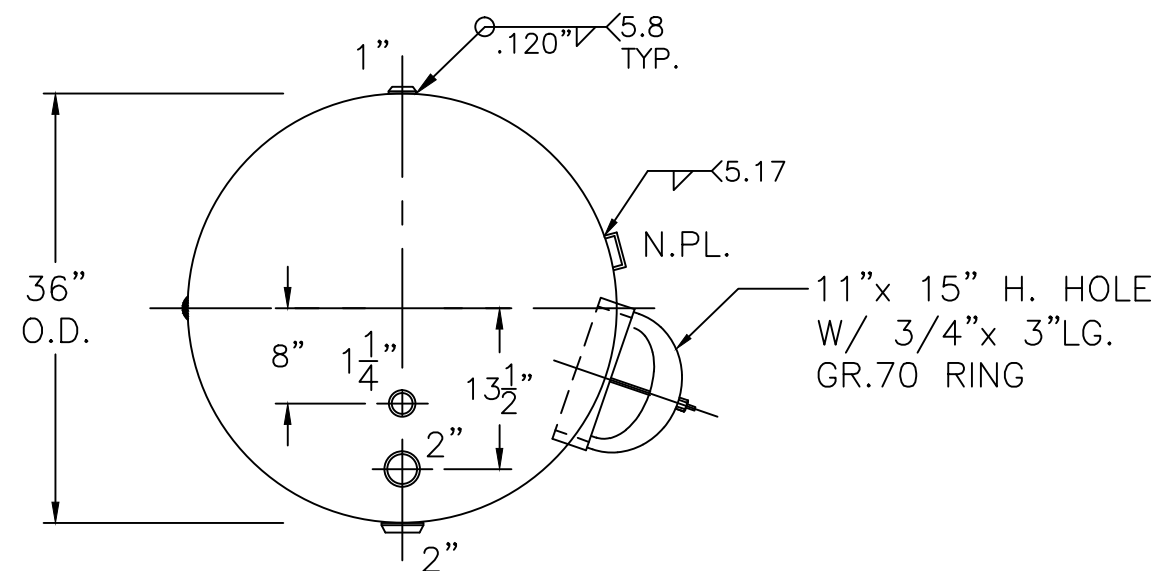
VIEW W/O SUPPORTS
