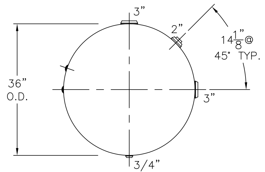
VIEW W/O SUPPORTS
